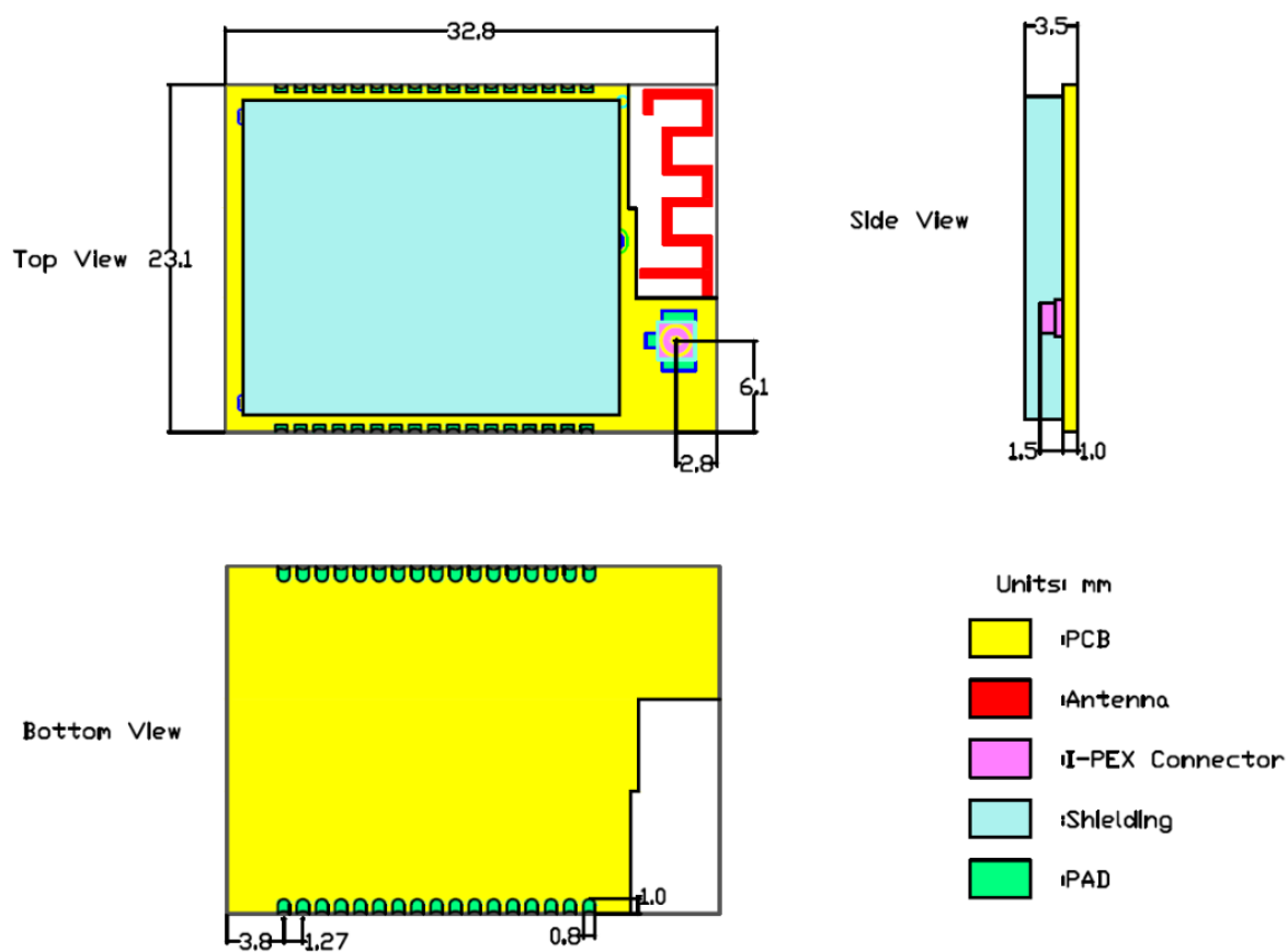
Figure 11. HF-LPB130 机械尺寸
