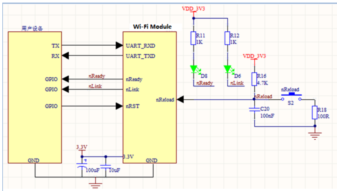
Figure 28. HF-LPX30 UART 应用硬件连接
