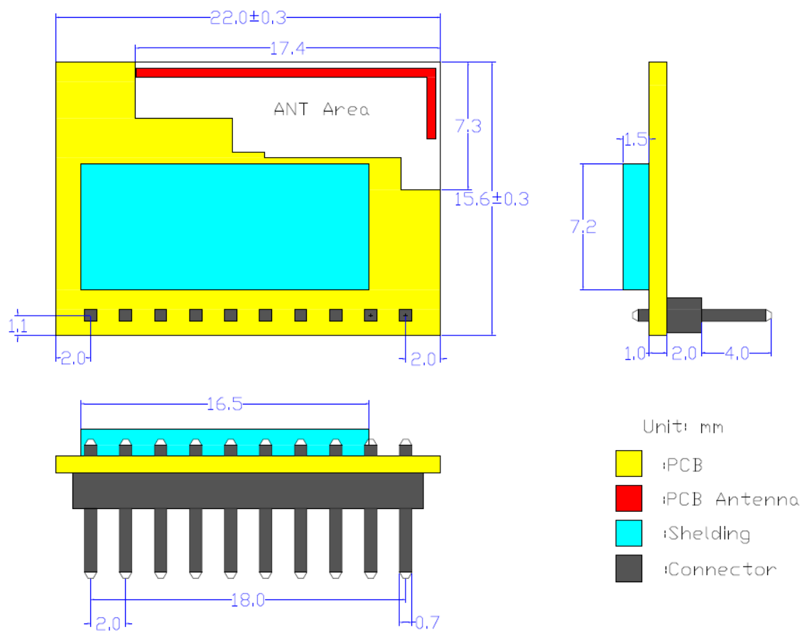
Figure 14. HF-LPT130B 机械尺寸
