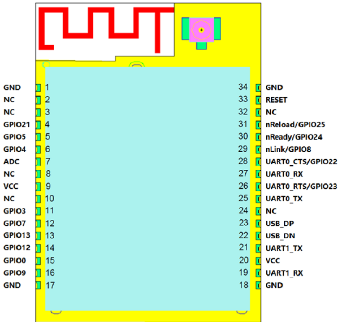
Figure 6. HF-LPB130 管脚定义
